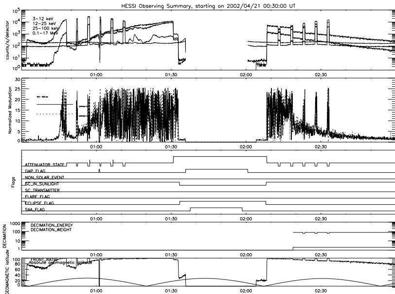
Figure 6. For each event, HEDC has an ‘Observing Summary page’, showing several products available in the Observing Summary, as well as RHESSI’s geomagnetic latitude. The usual color-coded version is available with the CD-ROM material accompanying this volume.
