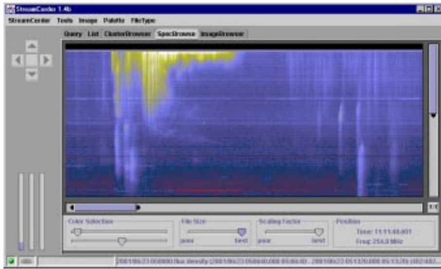
Figure 3. The StreamCorder is an alternative to the Web interface. It can search and display all HEDC data products. Here, it is displaying a wavelet-encoded radio spectrogram from Phoenix-2.
