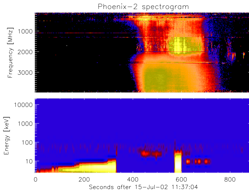
Figure 7. For each event, HEDC has a back-subtracted spectrogram from both RHESSI and Phoenix-2 radio data.
