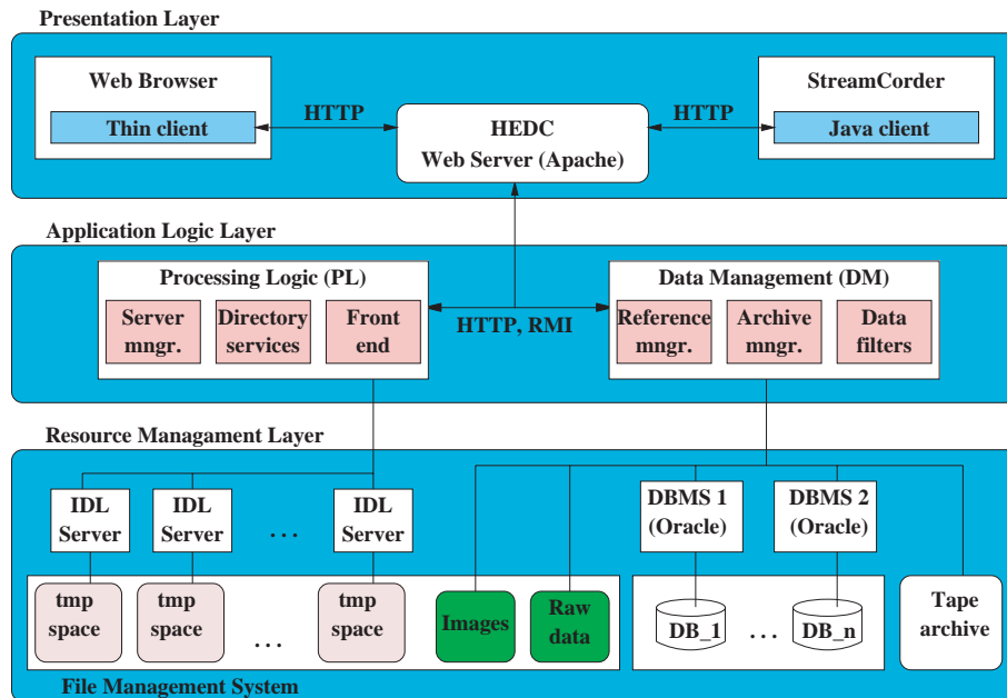
Figure 2. Architecture of HEDC
